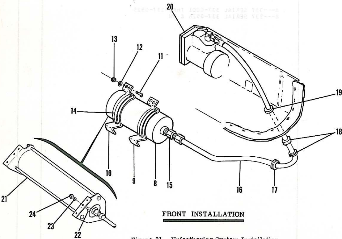
Figure 81. Unfeathering System Installation
