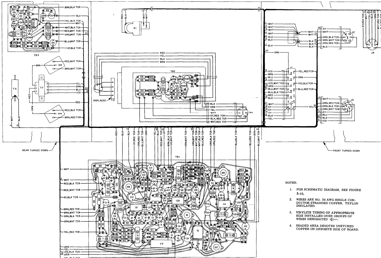
Figure 2-11. Computer Amplifier, Main Wiring Diagram
